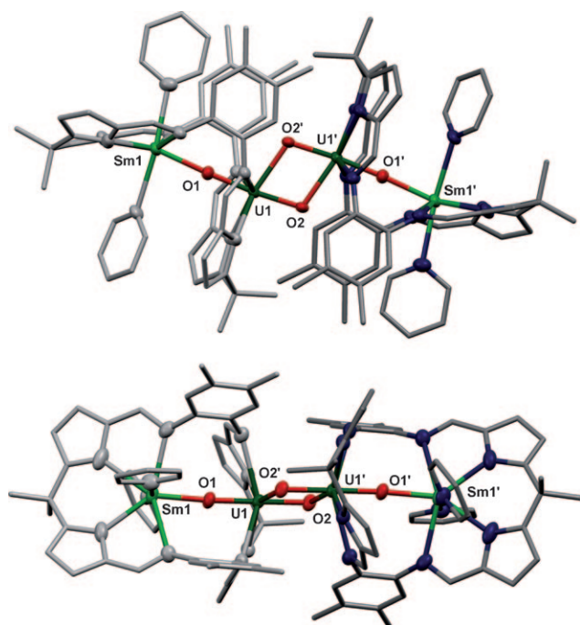
Figure 1. The solid-state structure of [\{UO_2Sm(py)_2(L)\}_2] ( 2 ). One molecule from the unit cell is shown, with hydrogen atoms and pyridine disorder components omitted (50% probability displacement ellipsoids where drawn).
