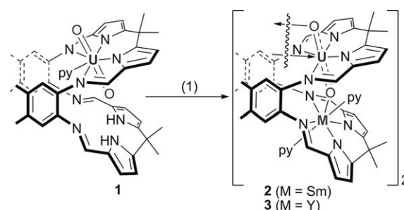
Scheme 1. Synthesis of uranyl–rare earth compounds of the macrocycle \text{H}_4\text{L} ( \text{M} = \text{Sm}, \text{Y} ). Reagents and conditions: 1) [\text{Sm}(\text{THF})_2[\text{N}(\text{SiMe}_3)_2]_2] , pyridine (py); or [\text{Y}[\text{N}(\text{SiMe}_3)_2]_3] , py.
